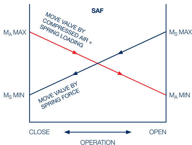
TORQUE CHARACTERISTIC OF TYPE SAF BR16 SINGLE ACTING ACTUATORS
